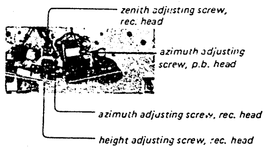
Fig. 4-3-3 Adjusting screws
